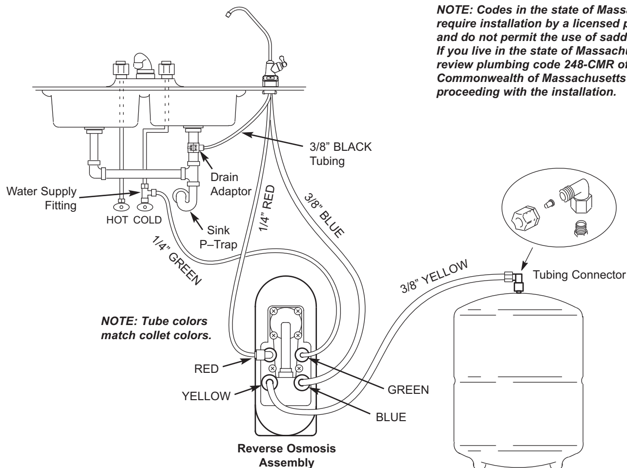
Tube Connections
